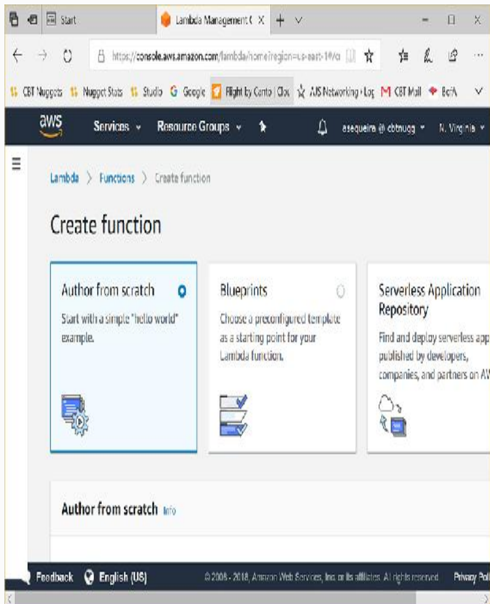
Figure 1-2 AWS Lambda
