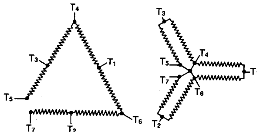
Fig. 8 - Open-Delta Constant-Horsepower Connection
