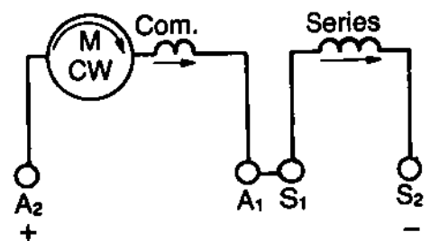
Fig. 12 - D-C Series-Wound Motor Connection for Clockwise Rotation
