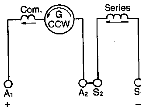
Fig. 18 - Series Generator Connection for Counterclockwise Rotation
