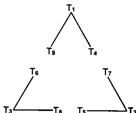
Fig. 25 – Standardized Lead Markings for Dual-Voltage Delta-Connected Windings
