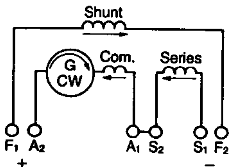
Fig. 19 - Compound Generator Connection for Standard Clockwise Rotation (also short shunt where A1, S2, S1, and F2 connect together and S1 is (-))
