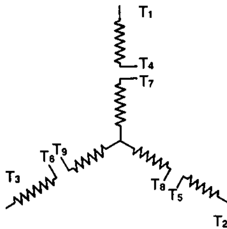
Fig. 1 - Dual-Voltage Three-Phase Star Connection
