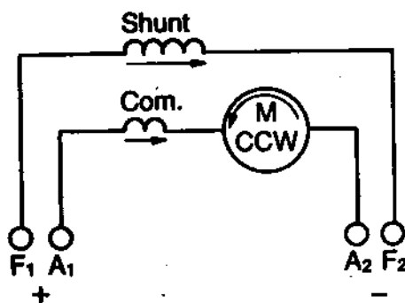
Fig. 9 - D-C Motor Connection for Standard Counterclockwise Rotation
