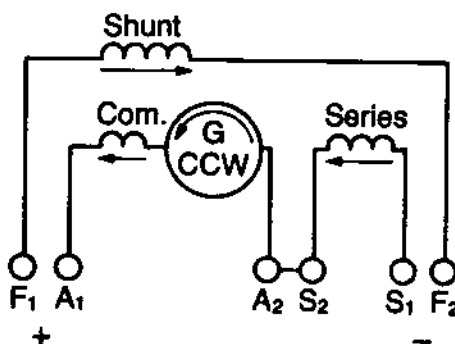
Fig. 20 - Compound Generator Connection for Counterclockwise Rotation (also short shunt, see Fig. 19)
