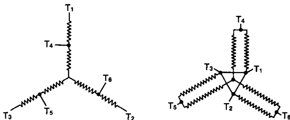
Fig. 4 - Two-Speed Variable-Torque Star Connected Motor
