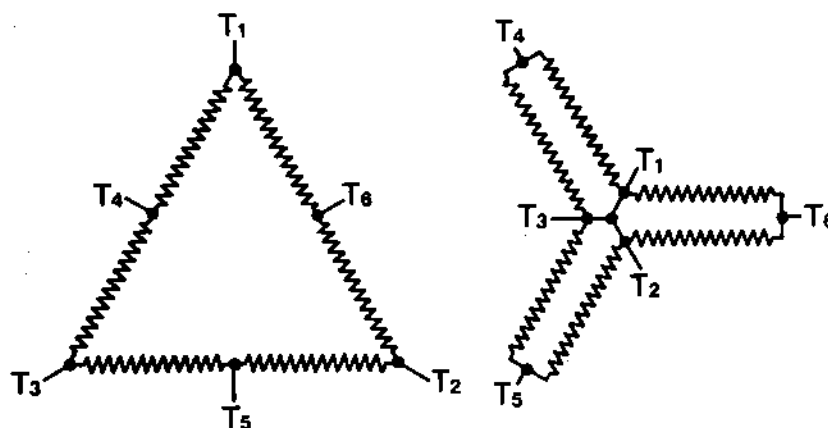
Fig. 5 – Two-Speed Constant-Torque Delta Connected Motor
