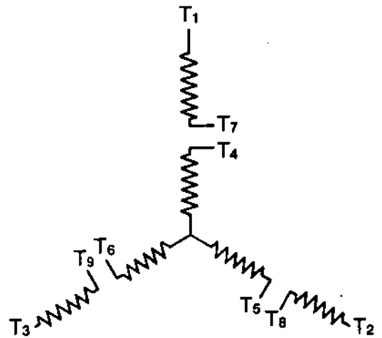
Fig. 1a - Dual-Voltage Star Connection (obsolete)
