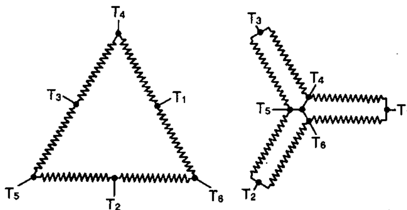
Fig. 6 - Delta Connected Motor for Constant-Horsepower
