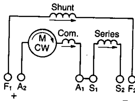
Fig. 14 - D-C Compound-Wound Motor Connection for Clockwise Rotation
