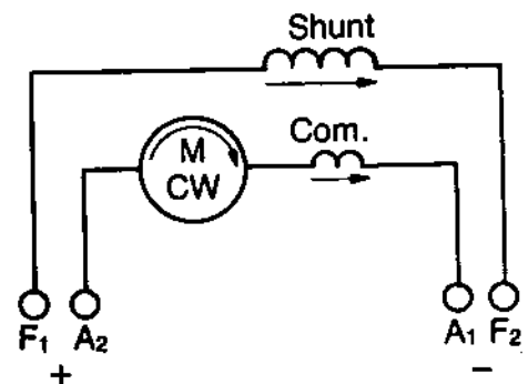
Fig. 10 - D-C Shunt-Wound Motor Connection for Clockwise Rotation
