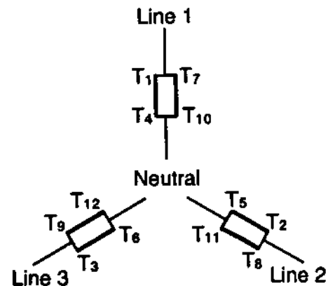
Fig. 22 – Typical Terminal Markings when All Terminal Circuit Leads are Brought Out
