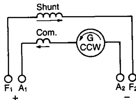
Fig. 16 - Shunt Generator Connection for Counterclockwise Rotation
