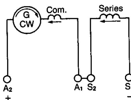
Fig. 17 - Series Generator Connection for Standard Clockwise Rotation
