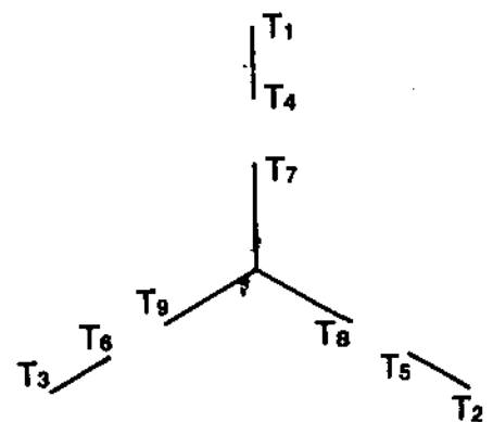
Fig. 24 – Terminal Markings when Nine Leads are Brought Out for Connection
