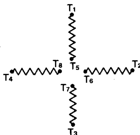
Fig. 3 – Two-Phase Double-Voltage Motor Connection
