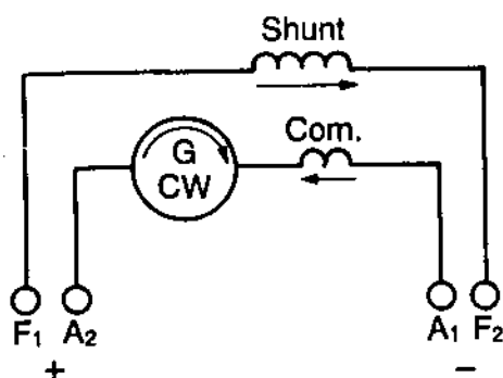
Fig. 15 - Shunt Generator Connection for Standard Clockwise Rotation
