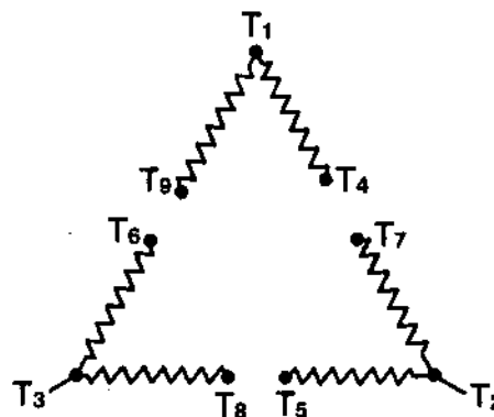
Fig. 2 - Dual-Voltage Three-Phase Delta Connection
